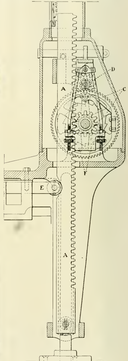
FIG. 3. MECHANICAL TIME LOCK
